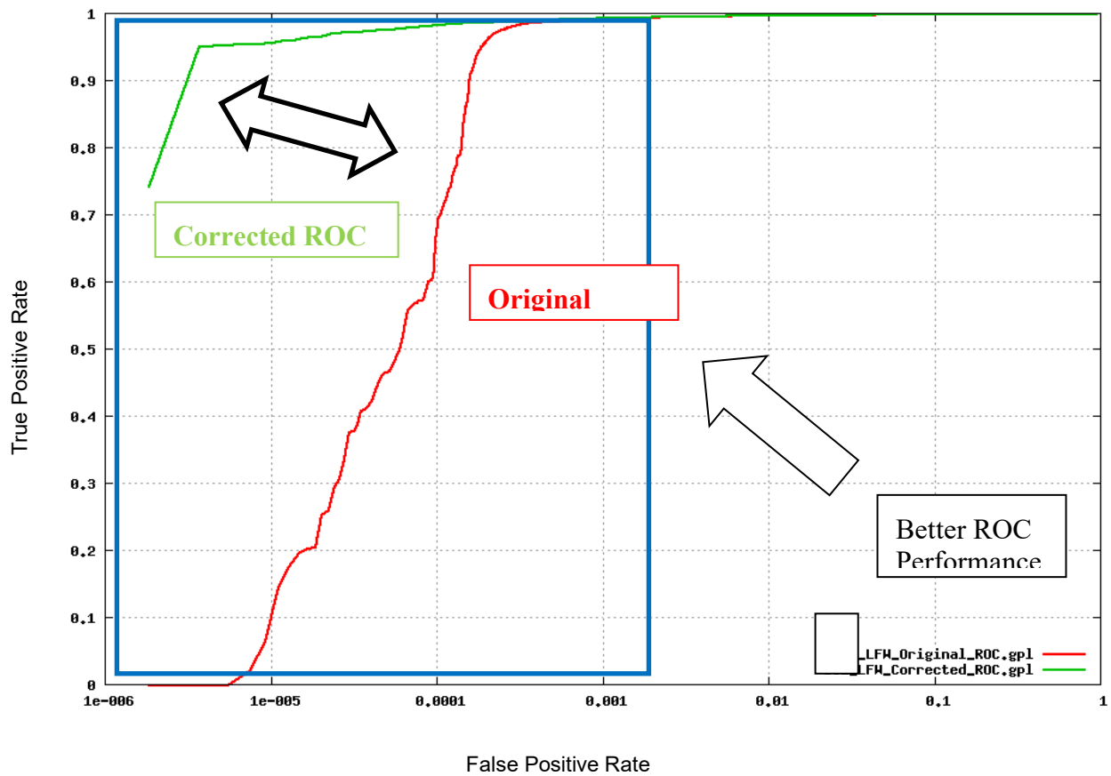
FIG. 8 ROC comparisons between original and corrected imagery
