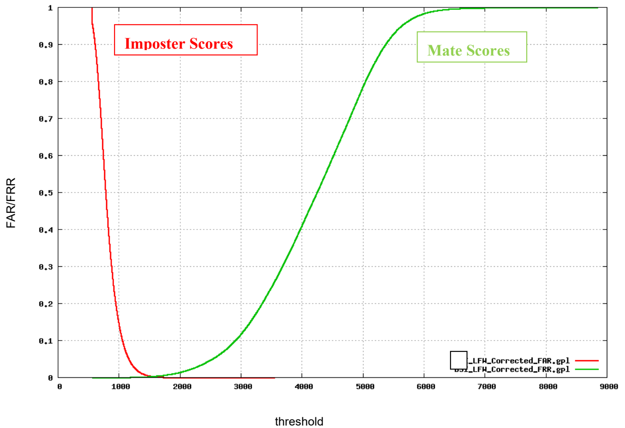
FIG. 3 FAR and FRR from corrected imagery
