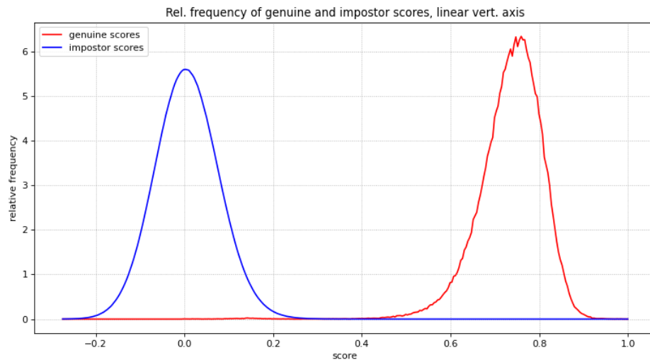
FIG. 12 Genuine and Imposter Scoring Histograms uncorrected imagery
