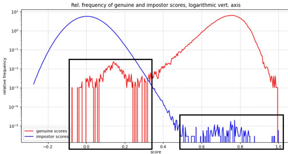
FIG. 13 Genuine and Imposter Scoring Histograms uncorrected imagery (Logr axis)
