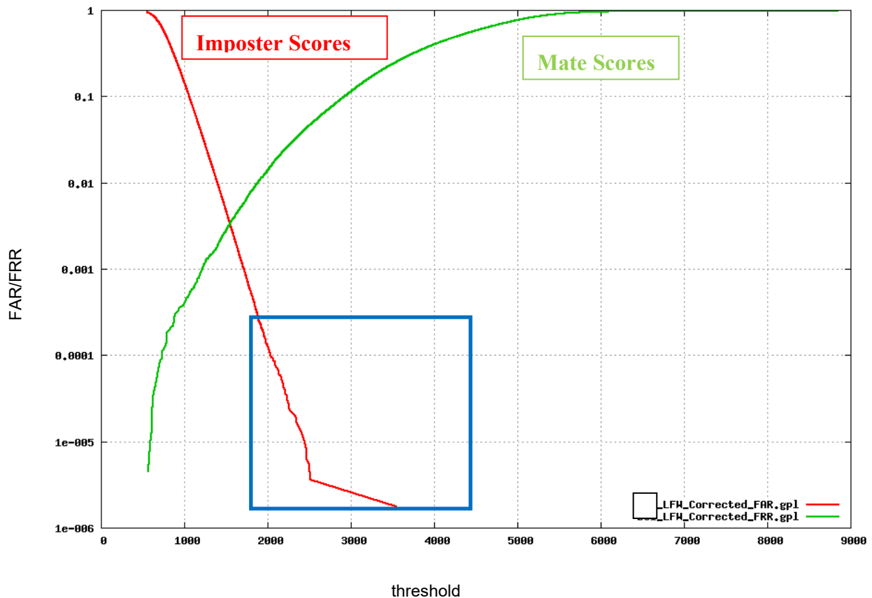
FIG. 4 FAR and FRR from uncorrected imagery
