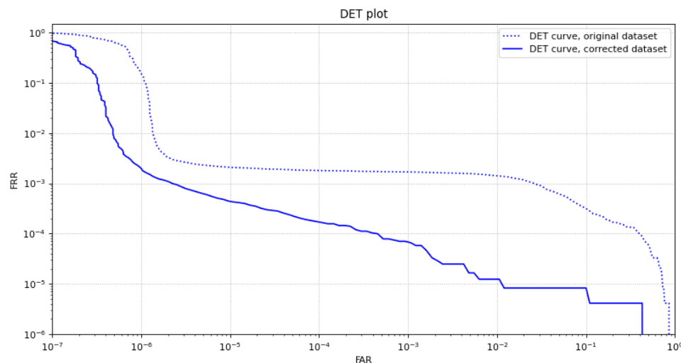
FIG. 17 DET from uncorrected/corrected imagery
