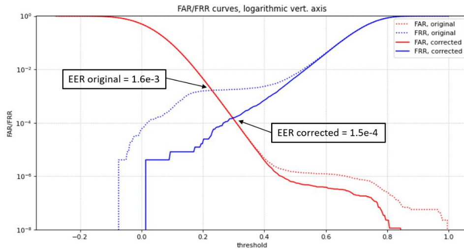
FIG. 16 FAR and FRR from uncorrected/corrected imagery (Logr axis)
