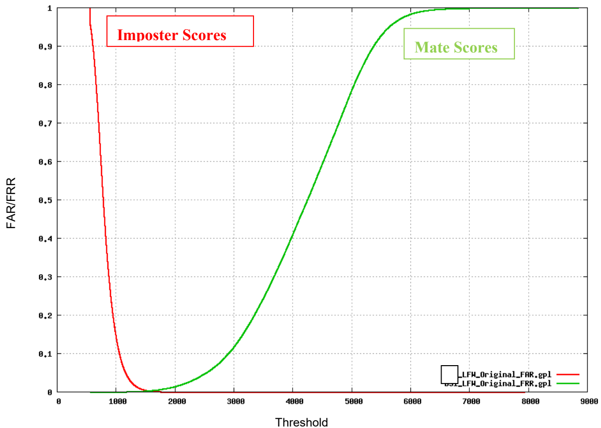
FIG. 1 FAR and FRR from uncorrected imagery
