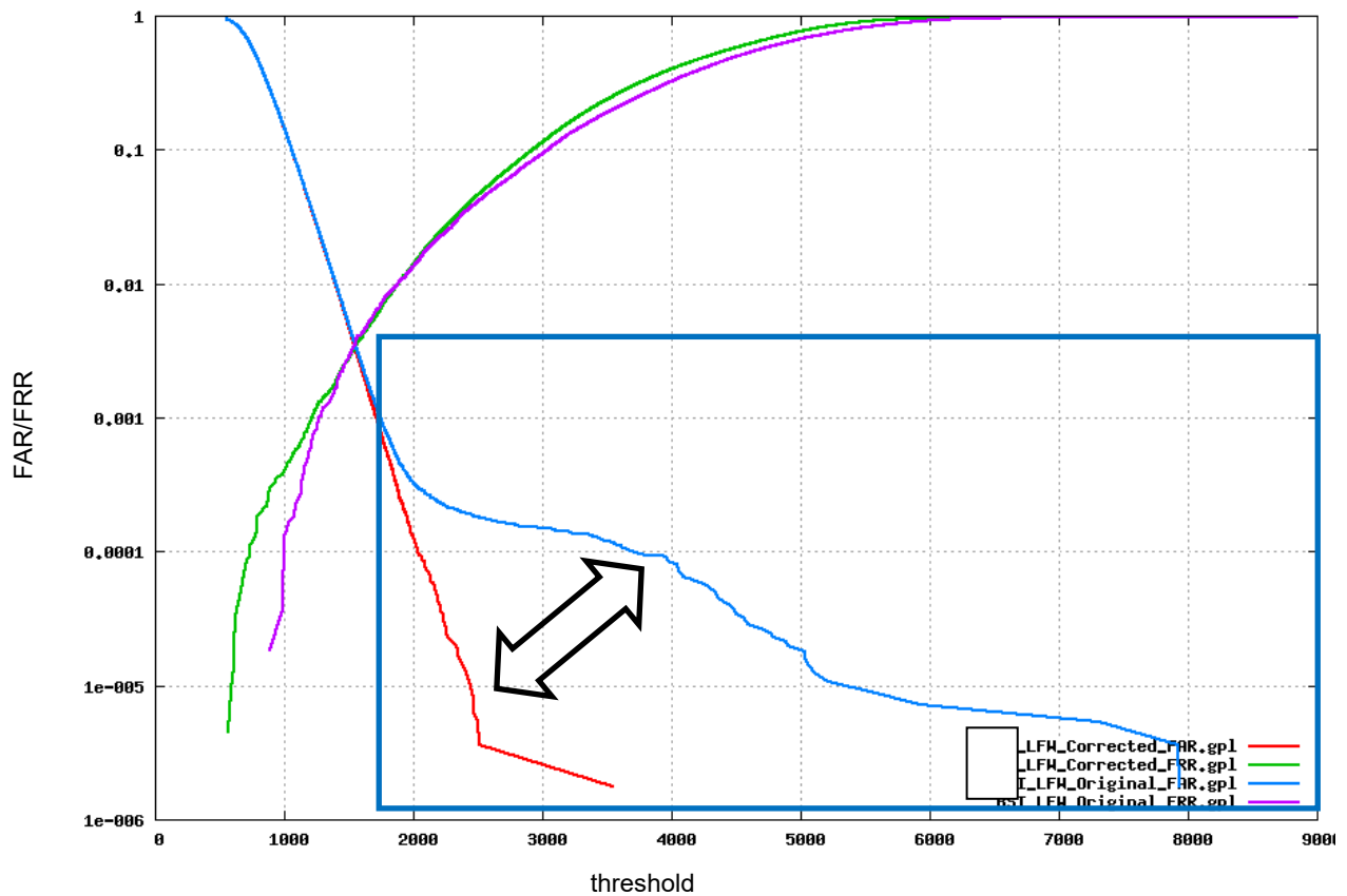
FIG. 6 FAR and FRR from original and corrected LFW imagery
