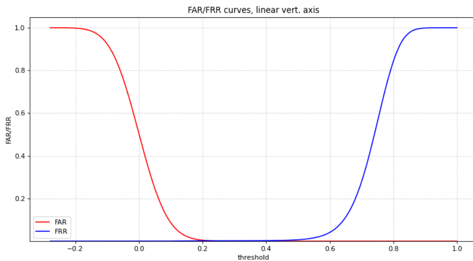
FIG. 10 FAR and FRR from uncorrected imagery
