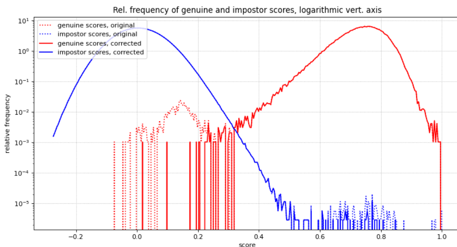
FIG. 15 Genuine and Imposter Scoring Histograms corrected imagery (Logr axis)
