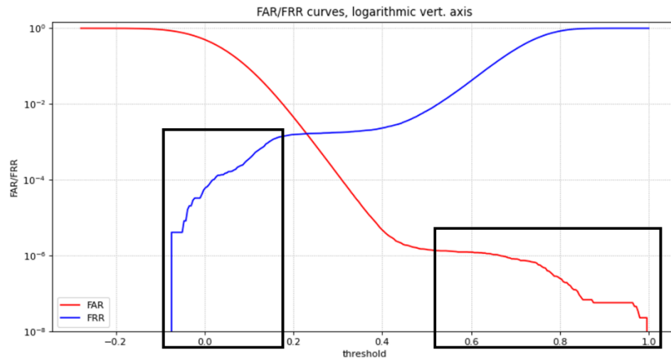
FIG. 11 FAR and FRR from uncorrected imagery (Logr axis)
