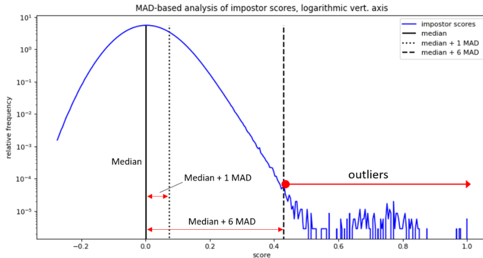
FIG. 14 MAD Based Imposter Scores uncorrected imagery (Logr axis)
