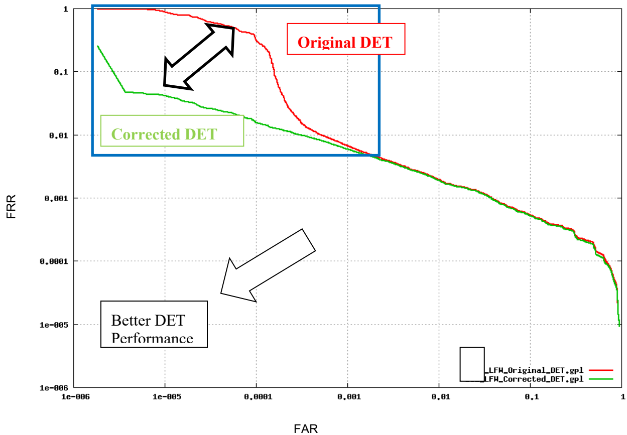
FIG 7 DET comparisons between original and corrected LFW imagery
