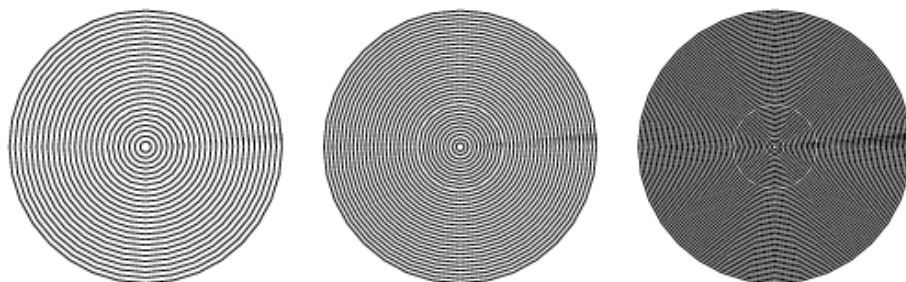
Figure 3: The illustrations above show a number of concentric circles plotted with a range of uniform spacing. Note the phantom lines and curves that appear. http://mathworld.wolfram.com/MoirePattern.html
